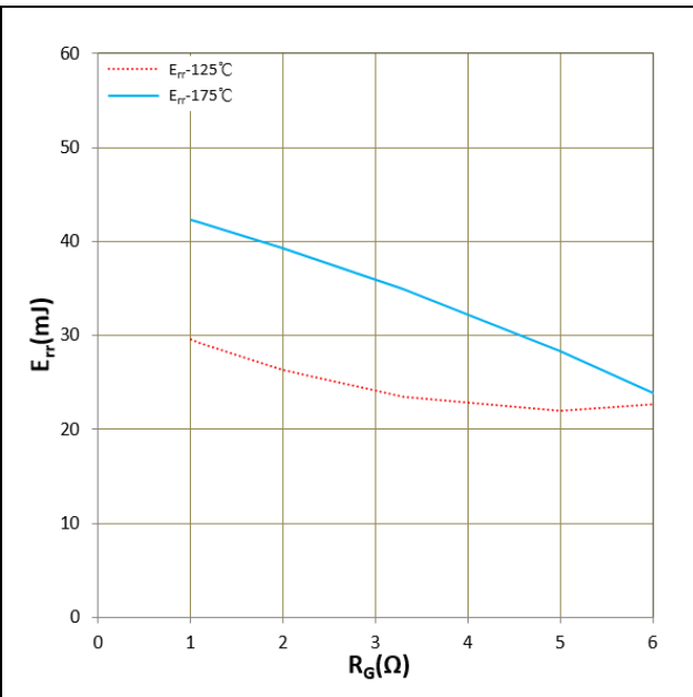
Figure 11. Err vs R_G (Typ) V_{CC}=600V , V_{GE}=+15V/-8V , I_F=900A Inductive Load
