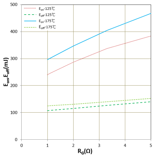
Figure 9. E_{on} , E_{off} vs R_G (Typ) V_{CC} = 600V , V_{GE} = +15V/-8V , I_c = 900A Inductive Load
