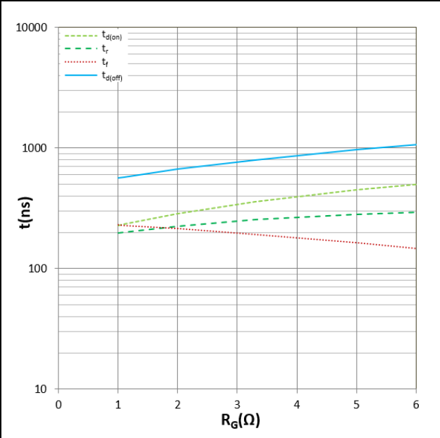
Figure 13. Switching time vs R_G (Typ) V_{CC}=600V , V_{GE}=+15V/-8V , I_C=900A T_j=175^\circ C , Inductive Load
