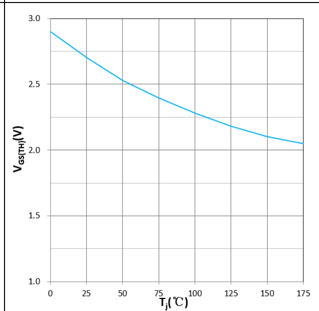
Figure 12. V_{GS(th)} vs T_j V_{GS}=V_{DS}, I_D=210mA
