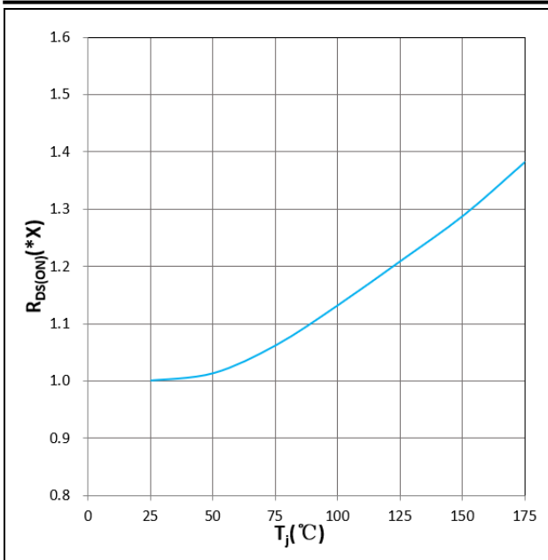
Figure 9. R_{DS(on)} vs T_j V_{GS}=+18V, I_D=600A, 1.0X=3.2m\Omega
