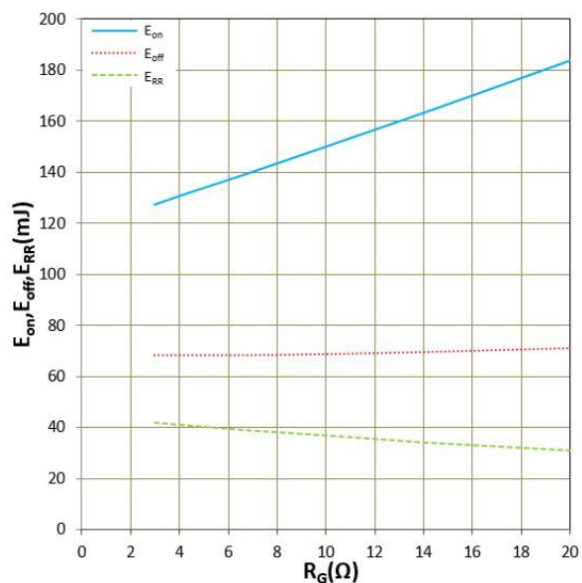
Figure 12. E on , E off , E rr vs R g (Typ)
