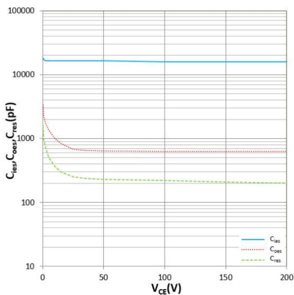
Figure 14. C ies , C oes , C res vs V CE
