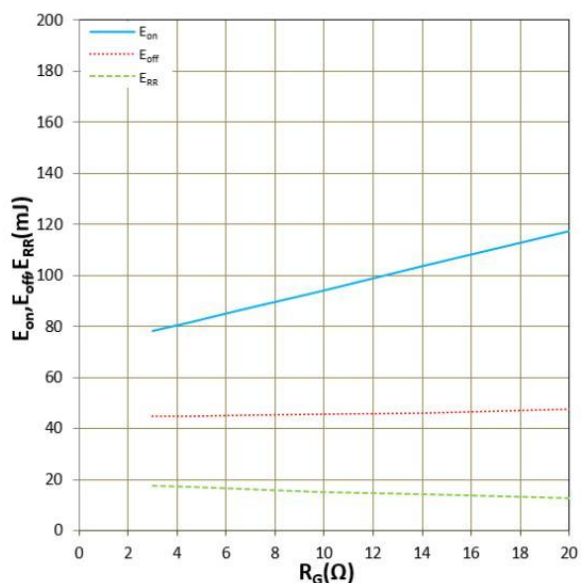
Figure 11. E on , E off , E rr vs R g (Typ)
