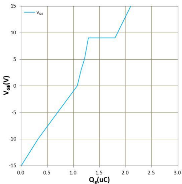
Figure 13. Gate charge
