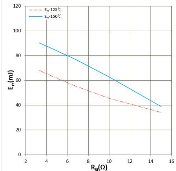
Figure 13. E_{rr} vs R_g (Typ) V_{CC}=900V , V_{GE}=+15V/-8V , I_F=450A Inductive Load
