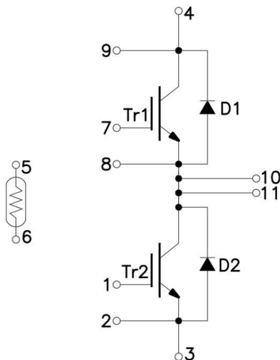
Figure 1. Out drawing & circuit diagram for DFI450HF17I4RE2
