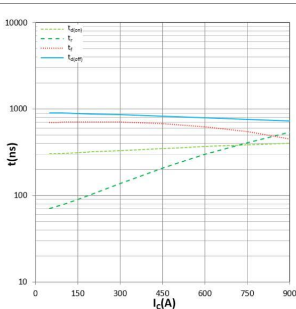
Figure 10. Switching time vs I_c (Typ)
