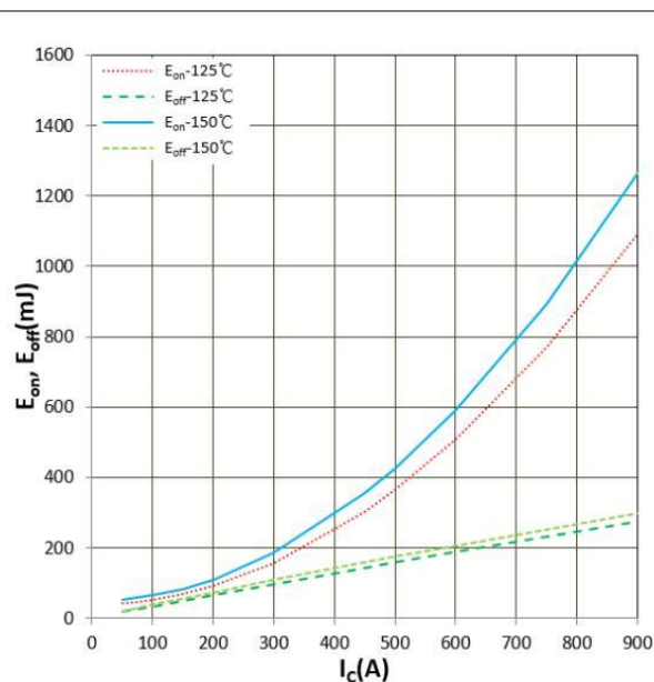
Figure 8. E_{on} , E_{off} vs I_c (Typ)
