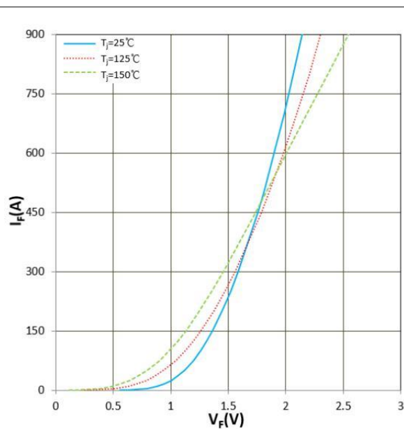
Figure 16. I_F vs V_F
