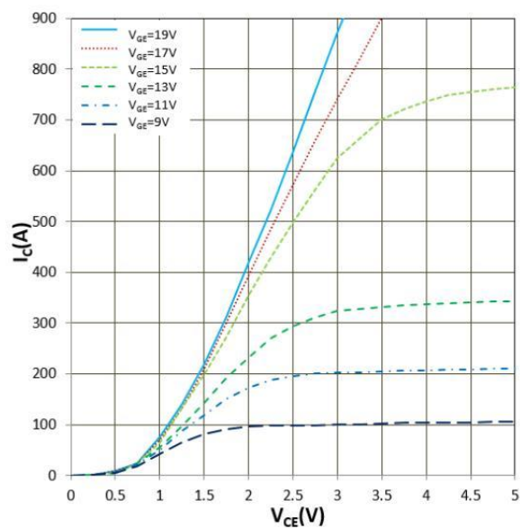
Figure 6. I_C vs V_{CE} T_j = 150^\circ C
