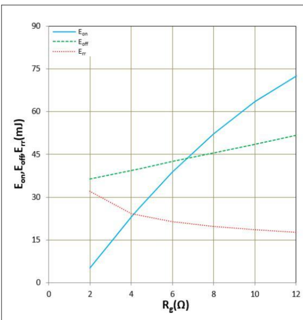
Figure 11. E_{on} , E_{off} , E_{rr} vs R_g (Typ) V_{CC}=600V , V_{GE}=+15V/-8V , I_C=300A , T_j=150^{\circ}C Inductive Load
