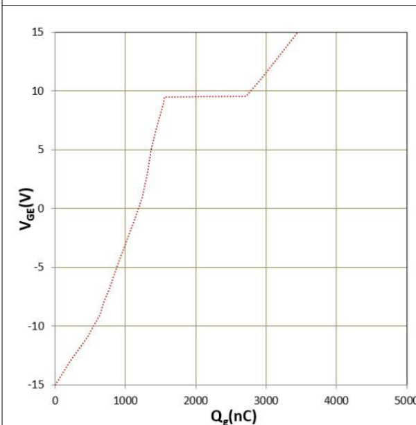
Figure 13. Gate charge
