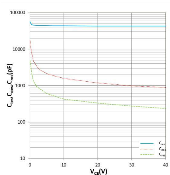
Figure 14. C_{ies} , C_{oes} , C_{res} vs V_{CE} T_j=25^{\circ}C , f=1MHz
