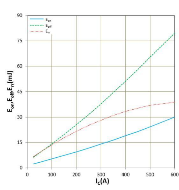
Figure 12. E_{on} , E_{off} , E_{rr} vs I_C (Typ) V_{CC}=600V , V_{GE}=+15V/-8V , R_g=3\Omega , T_j=150^{\circ}C Inductive Load
