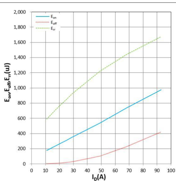
Figure 14. E_{on} , E_{off} , E_{rr} vs I_D
