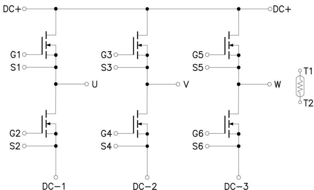
Figure 1. Out drawing & circuit diagram for DFS36FB14EYQ1
