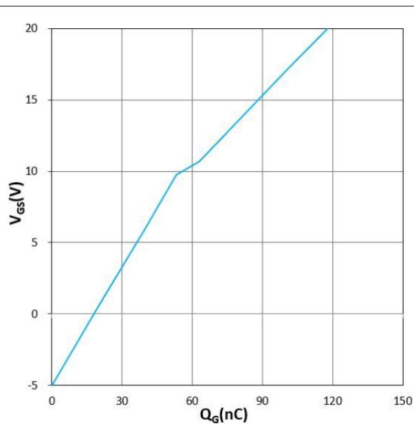
Figure 16. V_{GS} vs Q_G
