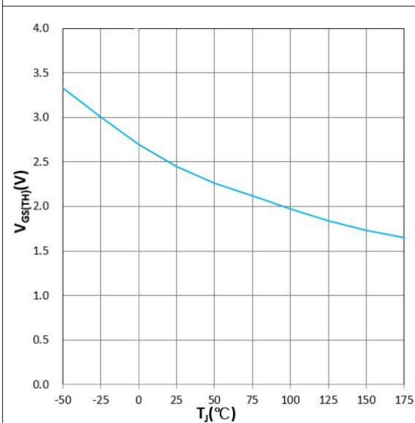
Figure 15. V_{GS(TH)} vs T_J
