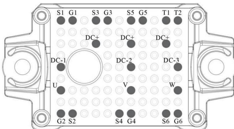
Figure 2. Pin configuration
