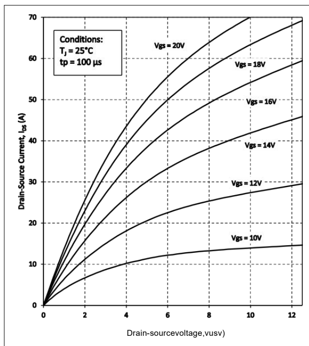
Figure 2. Output Characteristics T_j = 25^\circ\text{C}
