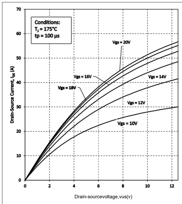
Figure 4. Output Characteristics T_j = 175^\circ\text{C}
