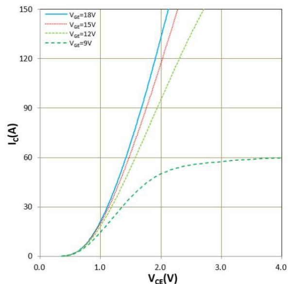
Figure 6. I_C vs V_{CE} T_J=175^{\circ}C
