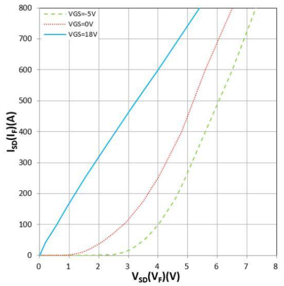
Figure 8. I_{SD}(I_F) vs V_{SD}(V_F)
