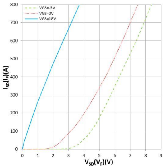
Figure 7. I_{SD}(I_F) vs V_{SD}(V_F)
