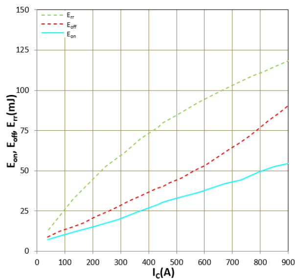
Figure 12. E_{on} , E_{off} , E_{rr} vs I_c (Typ) V_{CC}=600V , V_{GE}=+15V/-8V , R_g=1.2\Omega , T_j=150^\circ C Inductive Load
