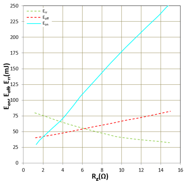
Figure 11. E_{on} , E_{off} , E_{rr} vs R_g (Typ) V_{CC}=600V , V_{GE}=+15V/-8V , I_C=450A , T_j=150^\circ C Inductive Load
