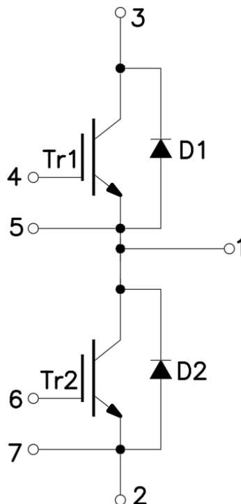
Figure 1. Out drawing & circuit diagram for DFI450HF12DFU1
