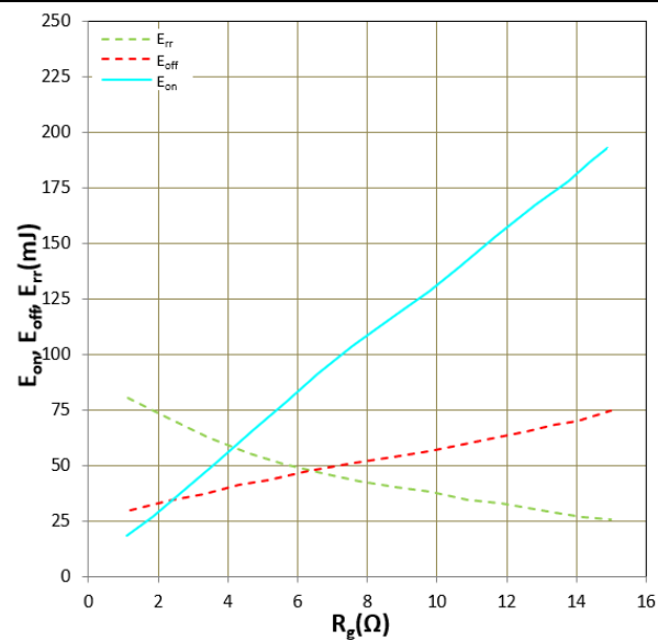
Figure 9. E_{on} , E_{off} , E_{tr} vs R_g (Typ) V_{CC}=600V , V_{GE}=+15V/-8V , I_c=450A , T_j=25^\circ C Inductive Load
