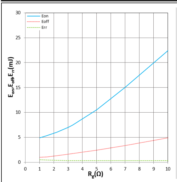
Figure 13. E_{on} , E_{off} , E_{rr} vs R_g T_j=25^\circ\text{C} , V_{DD}=600\text{V} , V_{GS}=+18\text{V}/-5\text{V} , I_D=300\text{A} Inductive Load
