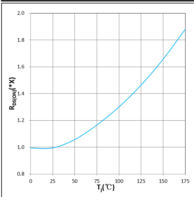
Figure 9. R_{DS(ON)} vs T_j V_{GS}=+20V, I_D=300A, 1.0X=6.6m\Omega
