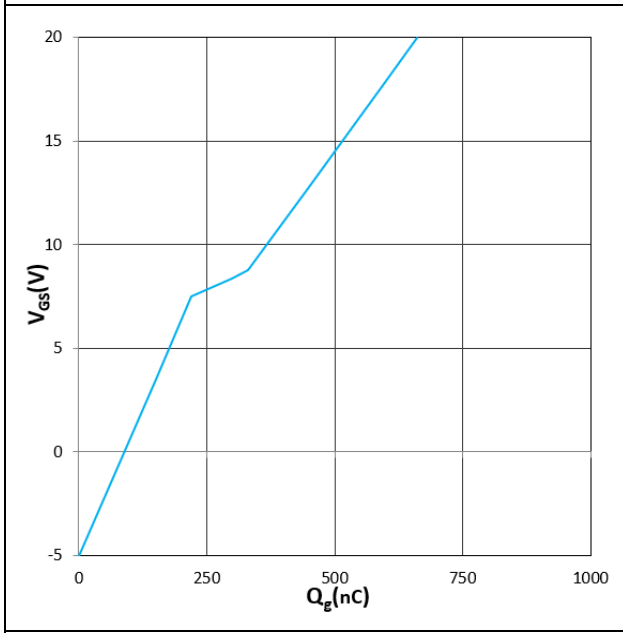
Figure 11. V_{GS} vs Q_g T_j=25^\circ C, V_{DS}=800V, I_D=150A
